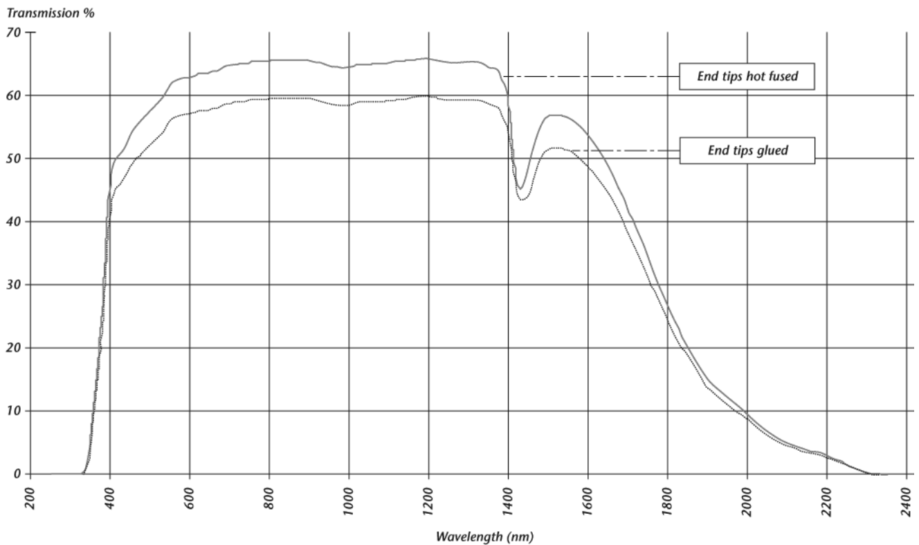
Spectral Transmission for 1 M Bundle, Fiber Type A2
